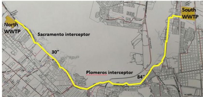
Figure 2 GRAVITY CONVEYANCE SYSTEM
